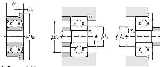
With flanged OR and double shield (FL...ZZ)
