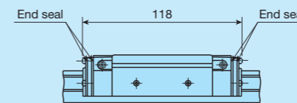
Fig. 2 Silde unit with double end seals (Size 25) (Supplemental code /V, /VV)
