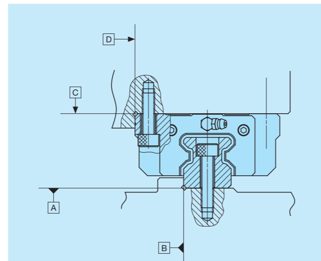
Fig. 5 Reference mounting surfaces and general mounting structure of Linear Way and Linear Roller Way
